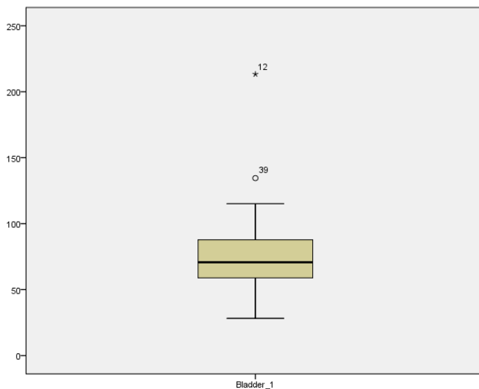
Figure 3. Boxplot of Bladder_1 volumes
